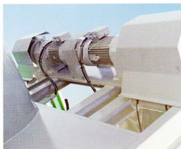
Two rope technology
